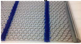
Self-cleaning Screens
